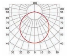
Low opal cover (light reduction: -31%)
