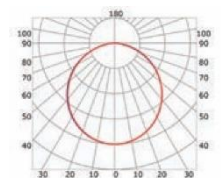
— C0-C180 — C90-C270 Flat opal cover (light reduction: -45%)
