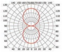
Flat opal cover (light reduction: -43%)
