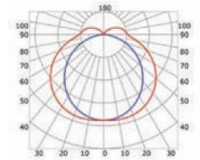
— C0-C180 — C90-C270 High opal cover (light reduction: -38%)
