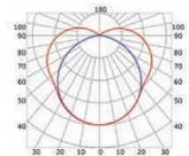
Opal L cover (light reduction: -25%)
