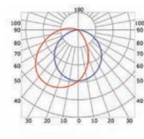
Opal cover (light reduction: -37%)
