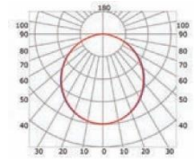
Opal cover (light reduction: -37%)
